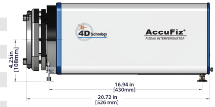
AccuFiz 4 in Aperture Model
